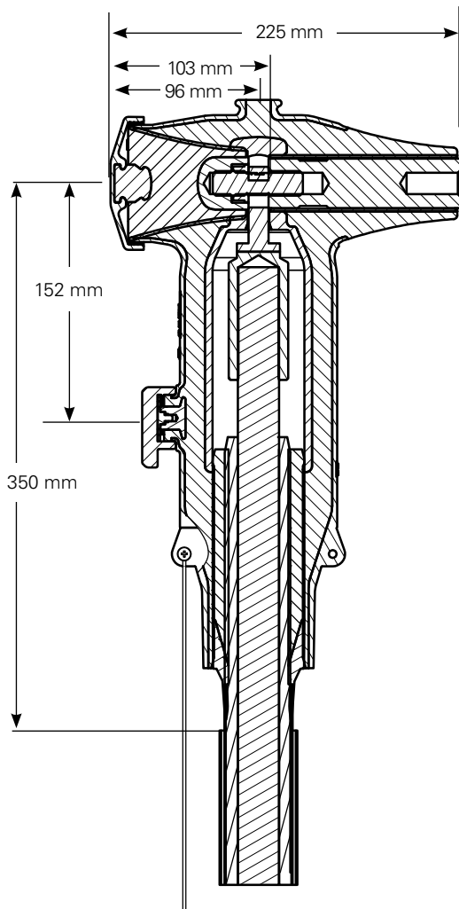
Figure 2. DTB1242 bolted companion tee connector dimensional information.
